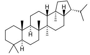
Triterpenoid
